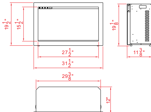
CLASSIC-SLIM-30
