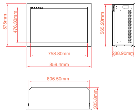
CLASSIC-33
