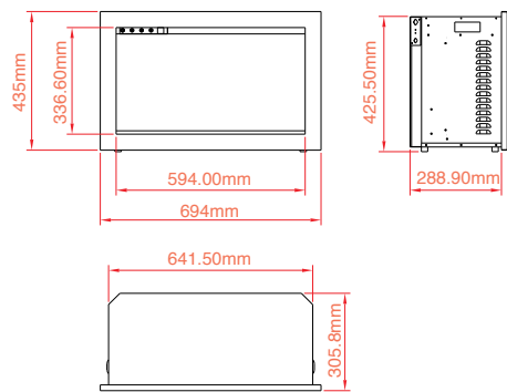
CLASSIC-26
