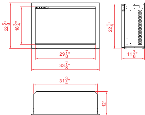
CLASSIC-SLIM-33
